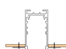
Cut out: W55mm, H90mm 开孔尺寸: 宽55mm, 高90mm
