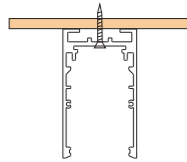
Surface mounted (明装)
