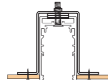
Cut out: W50mm, H120mm 开孔尺寸: 宽50mm, 高120mm
