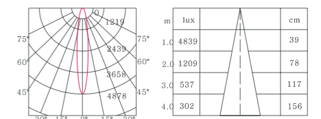
Beam Angle=24°
