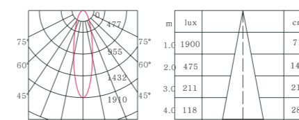
Beam Angle=36°
