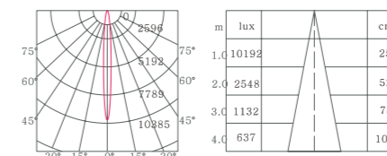
Beam Angle=15°
